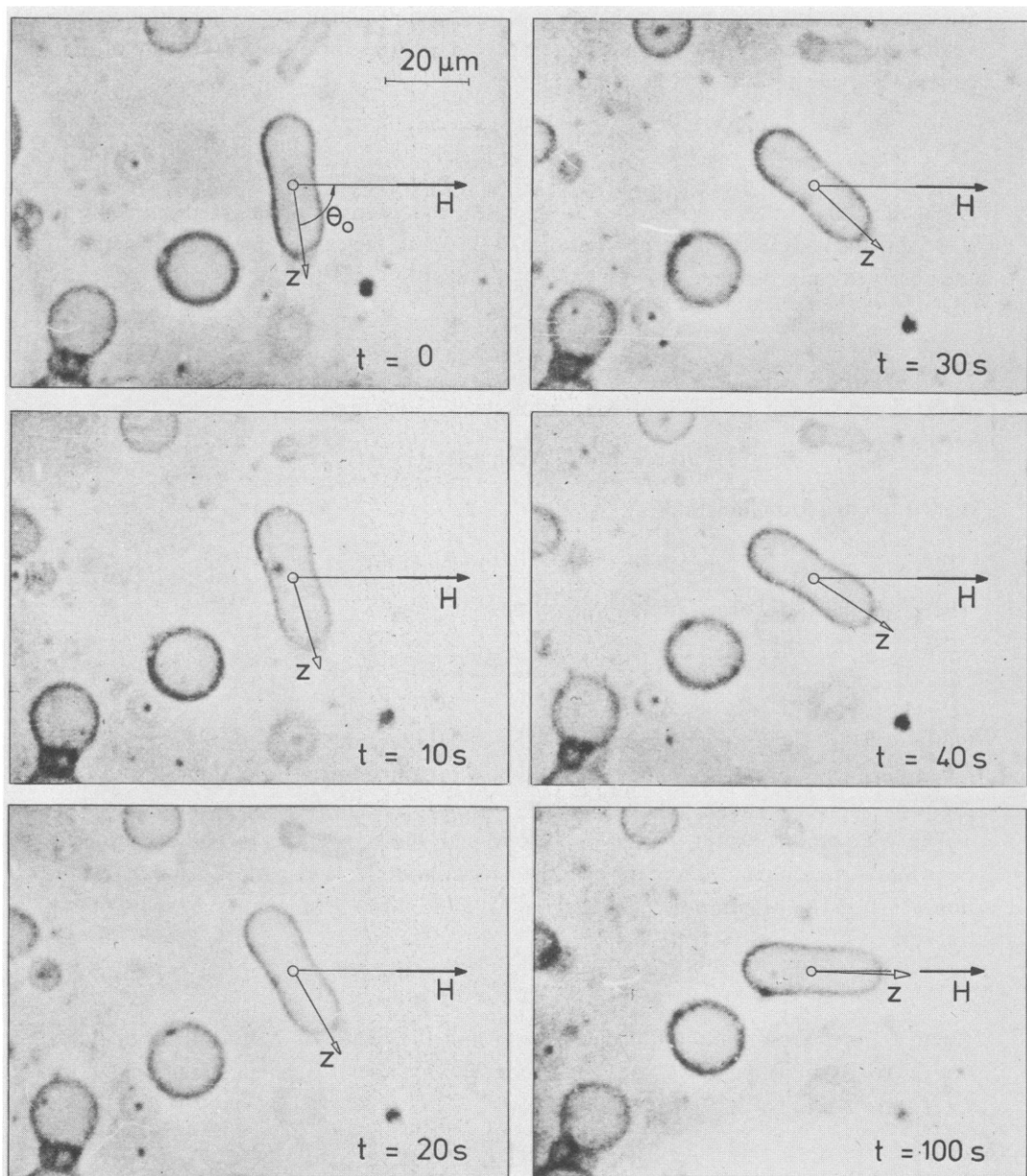
FIGURE 1 Time sequence of alignments of a cylindrical vesicle in a magnetic field, H .
